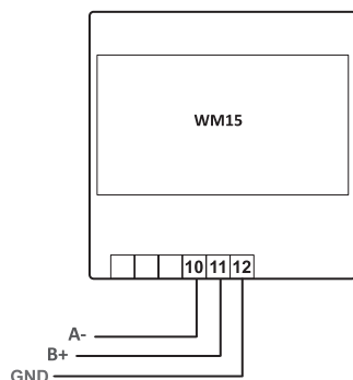
Abb. 14 RS485-Port
